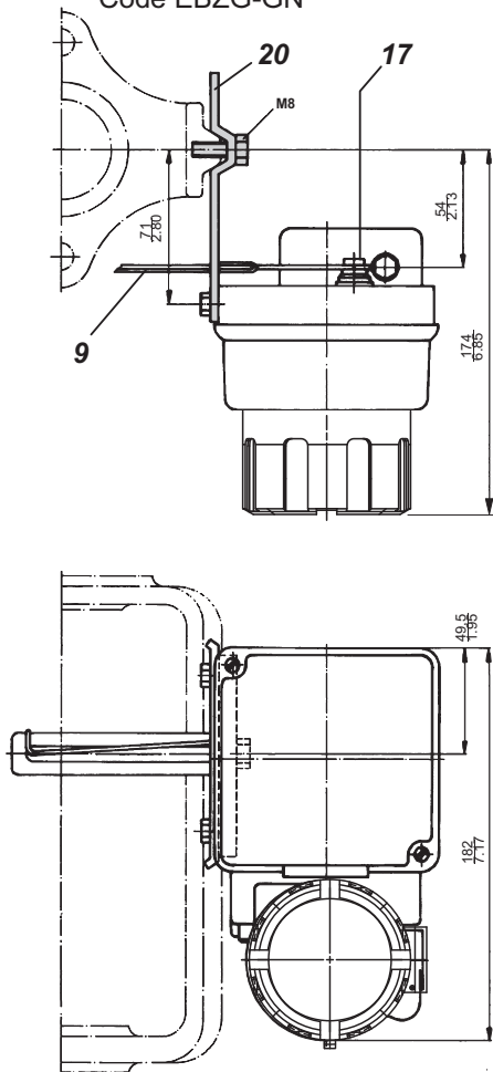
Attachment to casting yoke according to IEC 534-6 (NAMUR) Code EBZG-GN
